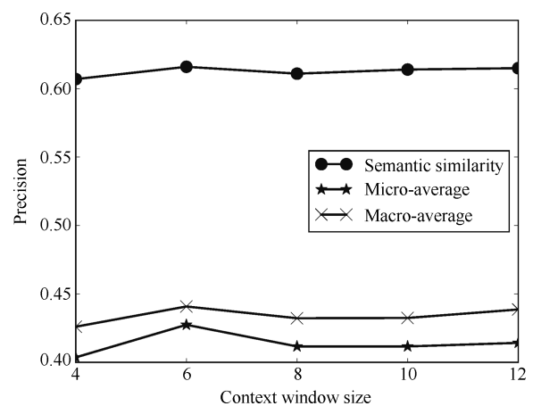
图 4 词义消歧精度和语义相似度精度与上下文窗口的关系 Fig. 4 The precisions of WSD and semantic similarity at different context window sizes
