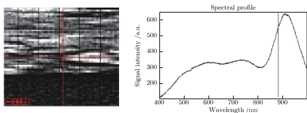
(a) 潜在缺陷点定位及频谱图 (a) Location of potential defects and spectrogram
