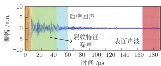
(b) 凝固裂纹的超声反射归一化信号 (b) Ultrasonic reflection normalized signal of solidification crack
