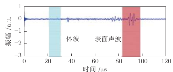
(a) 凝固裂纹的超声透射归一化信号 (a) Ultrasonic transmission normalized signal of solidification crack
