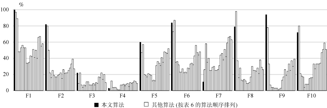
图 6 成功运行百分比柱状图 Fig. 6 Histogram of successful running percentage
