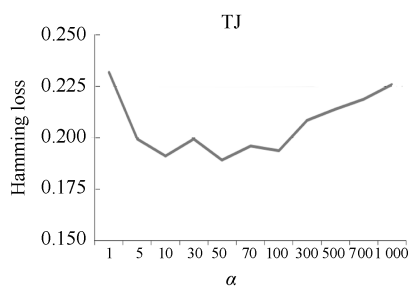
(a1) Hamming loss 值 (a1) Hamming loss value
