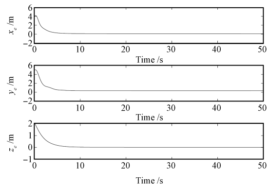
Fig. 7 Tracking errors of the closed-loop system without saturated control (Transient performances are better.)
