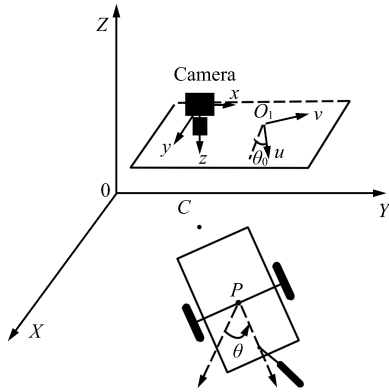
Fig. 2 Wheeled mobile robots with monocular camera
