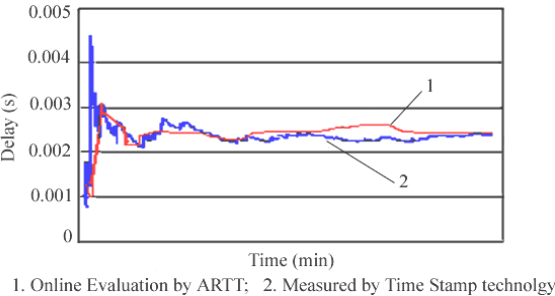
图 3 网络诱导时延 Fig. 3 Average of Ethernet delay online evaluation by different technology
