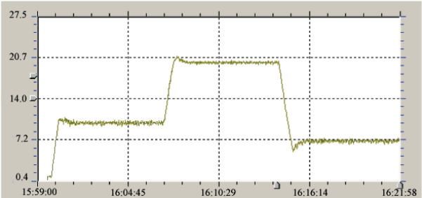
图 2 实验结果 Fig. 2 The experimental result based on delay on-line evaluation using ARTT
