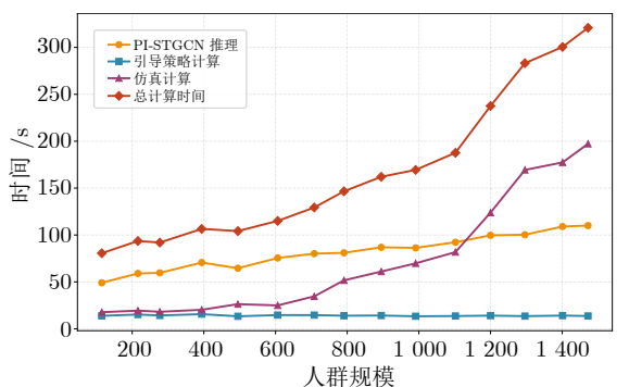
(a) 时间花费变化 (a) Variation of time cost
