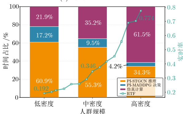
(b) 时间花费占比与实时率变化 (b) Variation of time cost proportion and real-time rate
