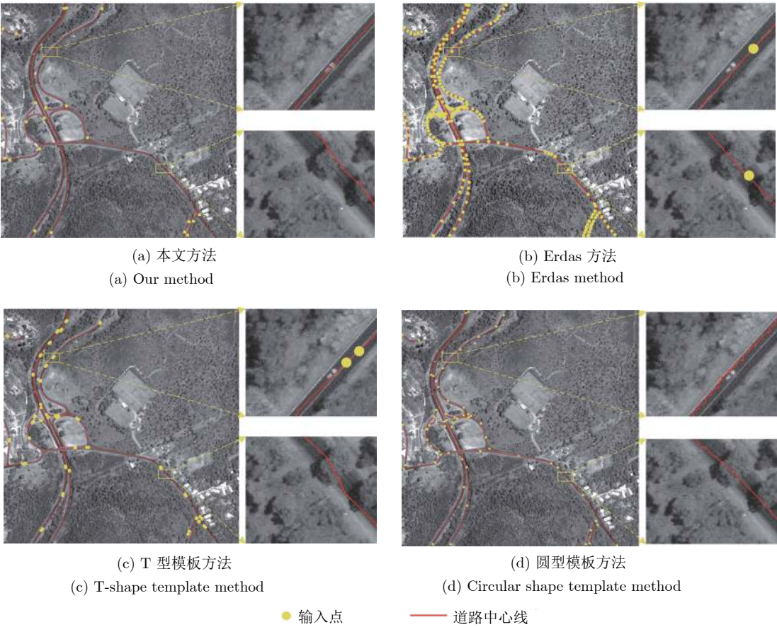
图 10 Geoeye-1 影像道路中心线提取 Fig.10 Road centerline extracted for Geoeye-1 image
