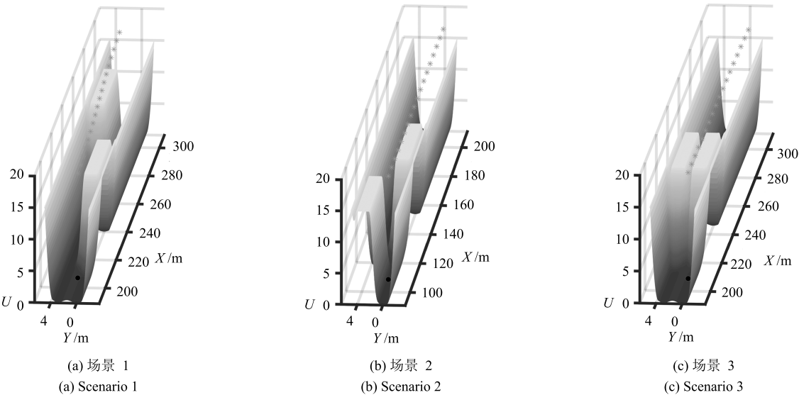
图 6 各场景关键时刻势场分布图 Fig. 6 Potential distributions at key moments in several scenarios
