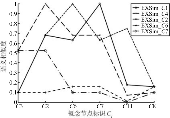
图 4 EXSim [7] 所得不再同一分支的概念间相似度 Fig.4 Similarities between concepts at different branches by EXSim
