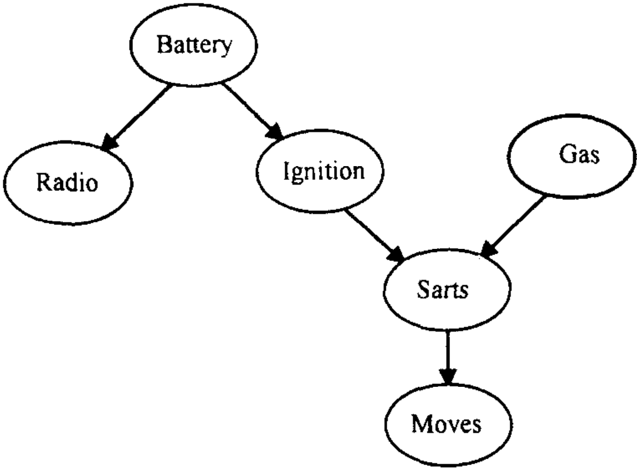
Fig.3 The Bayesian Network for car electric and engine system
