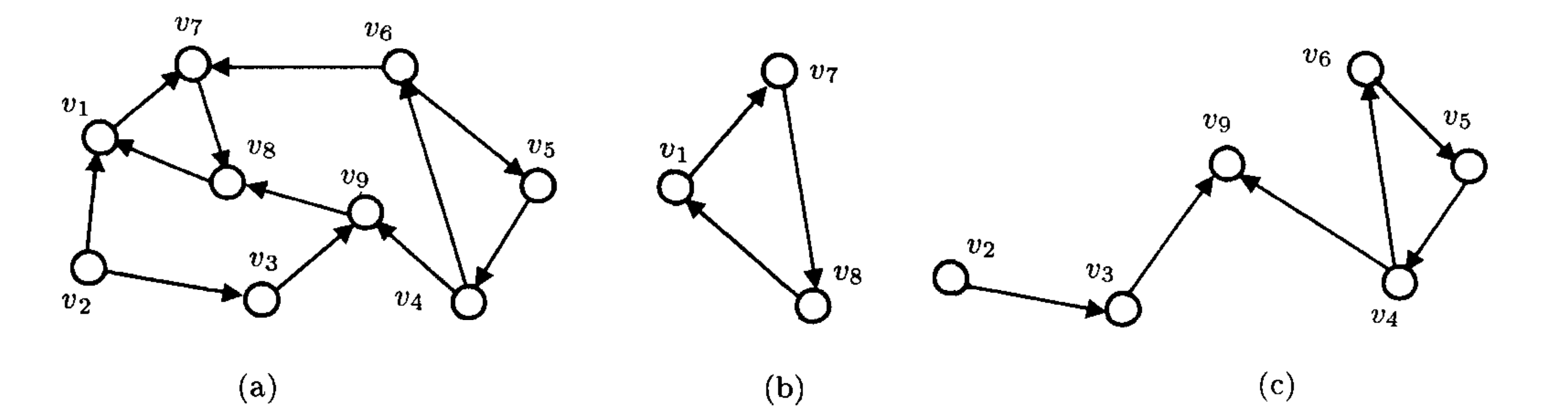
Fig.8 Regularly divided and basic FCMs: according to vertex v_9 , FCM in (a) is divided as Out(v_9) in (b) and In(v_9) in (c)
