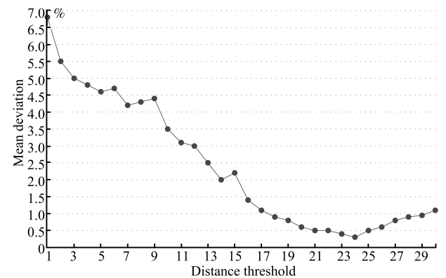
图 4 距离阈值对解质量的影响 Fig. 4 Influence on solution quality of distance threshold
